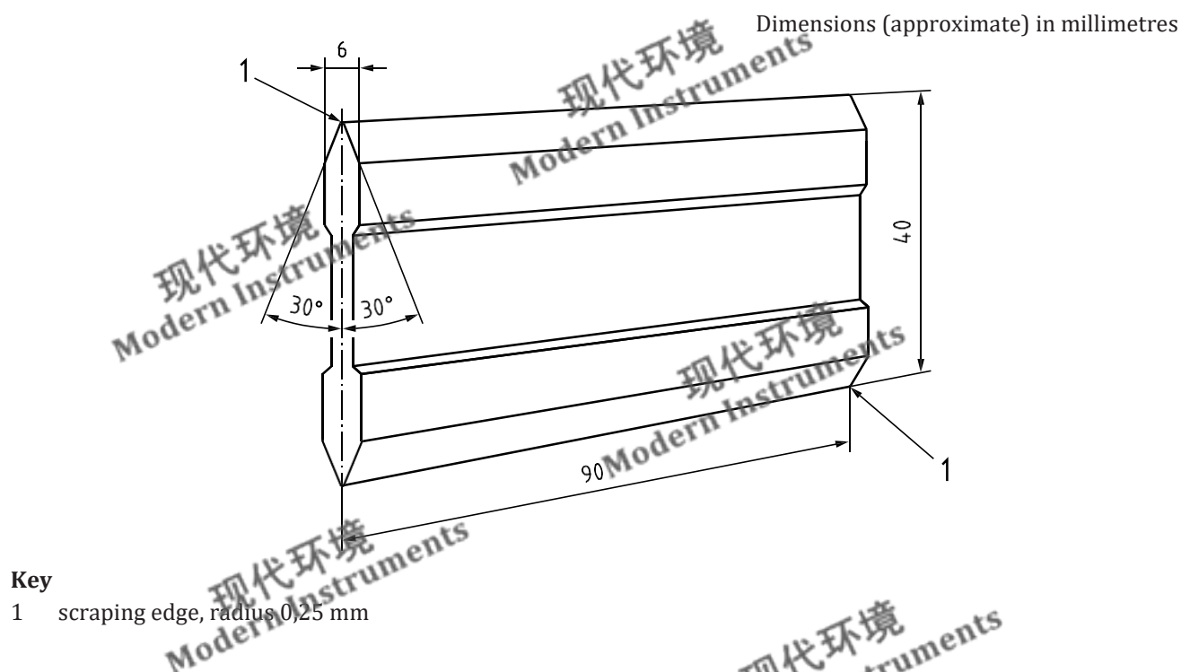
Figure 2 — Suitable scraper
