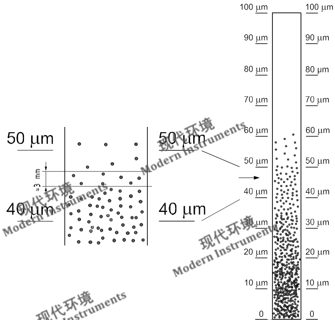
Figure 3 — Example of a gauge reading 45 μm
